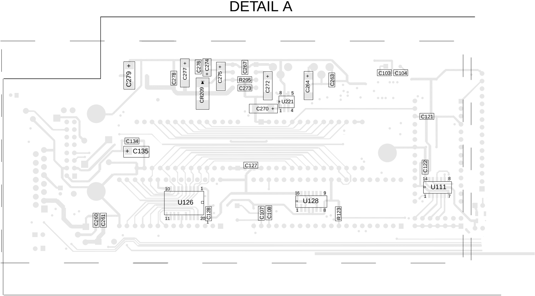
CVR INTERFACE BOARD COMPONENT LAYOUT (OPPOSITE COMPONENT SIDE) FIGURE 6-2 6-8
