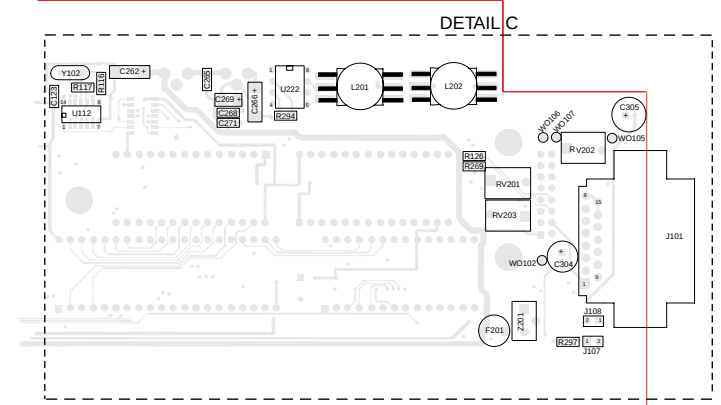
CVR INTERFACE BOARD COMPONENT LAYOUT (COMPONENT SIDE) FIGURE 6-1
