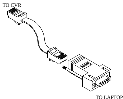
Figure 2-25 LAPTOP INTERCONNECT CABLE
