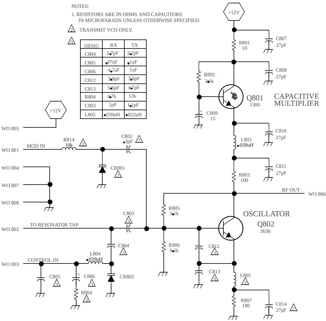
Figure 10-19 TRANSMIT VCO SCHEMATIC
