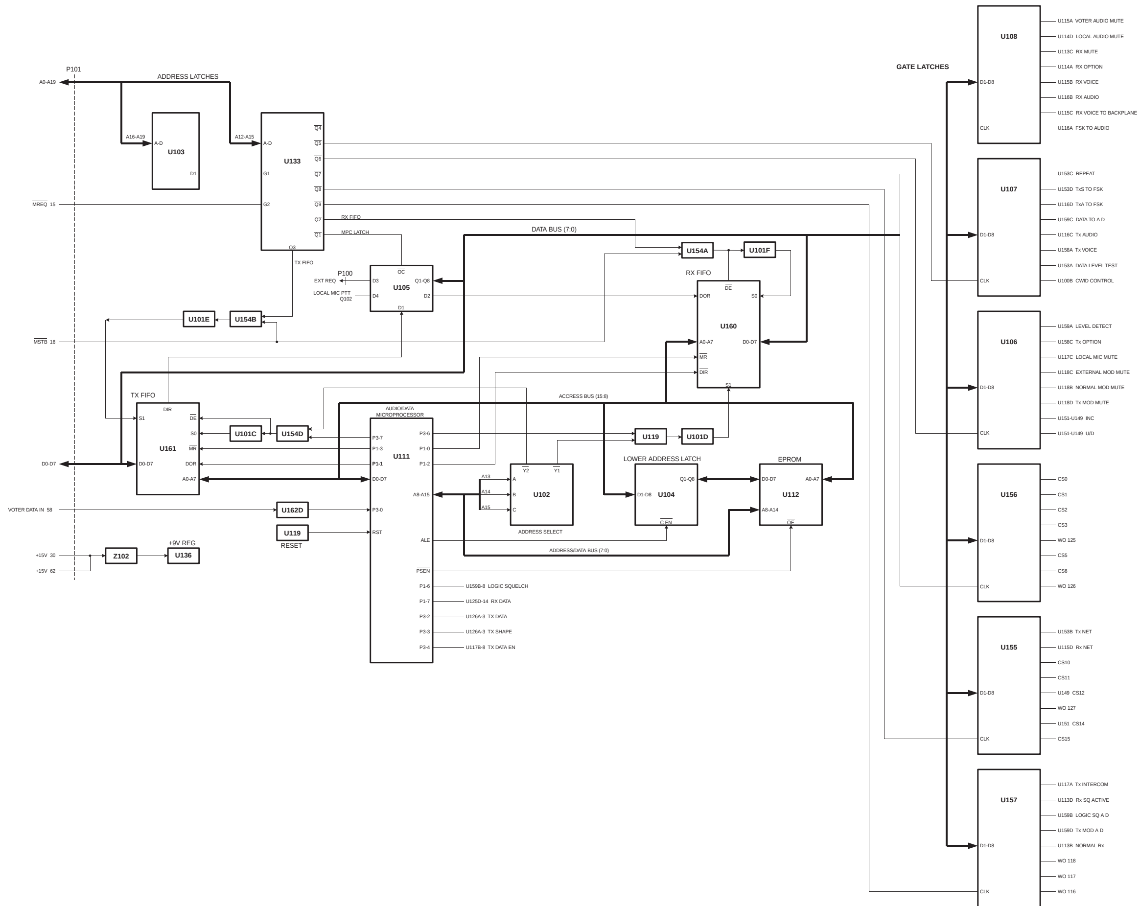
MAIN AUDIO CARD LOGIC BLOCK DIAGRAM FIGURE 6-21
