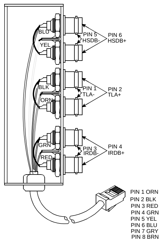
Figure 2-7 ANTENNA CONNECTIONS
