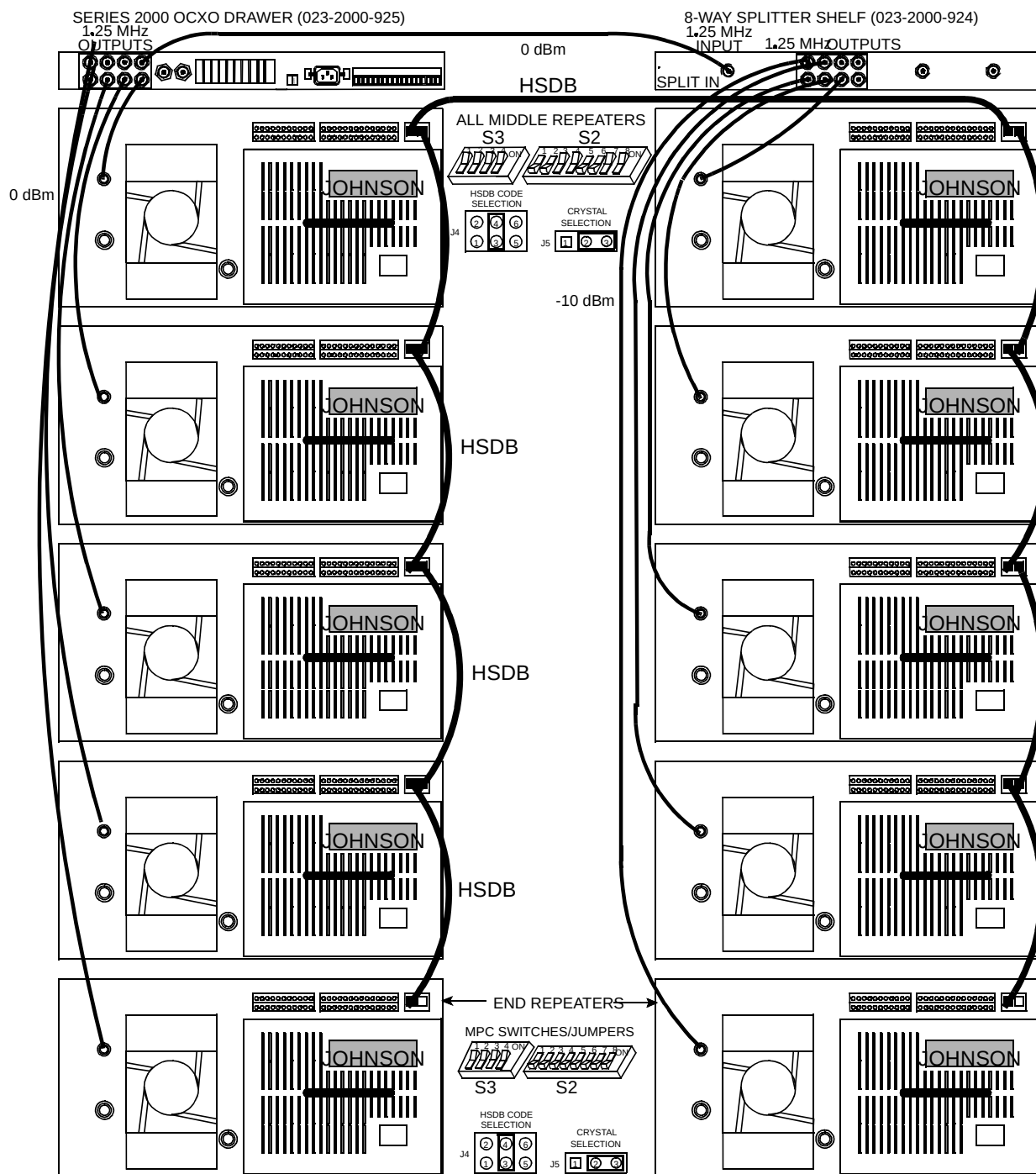
Figure 2-10 VIKING VX REPEATERS WITH 2000 OCXO DRAWER
