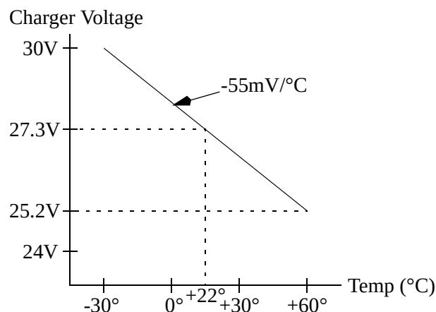
Figure 6-12 NO LOAD CHARGE VOLTAGE vs. TEMPERATURE
