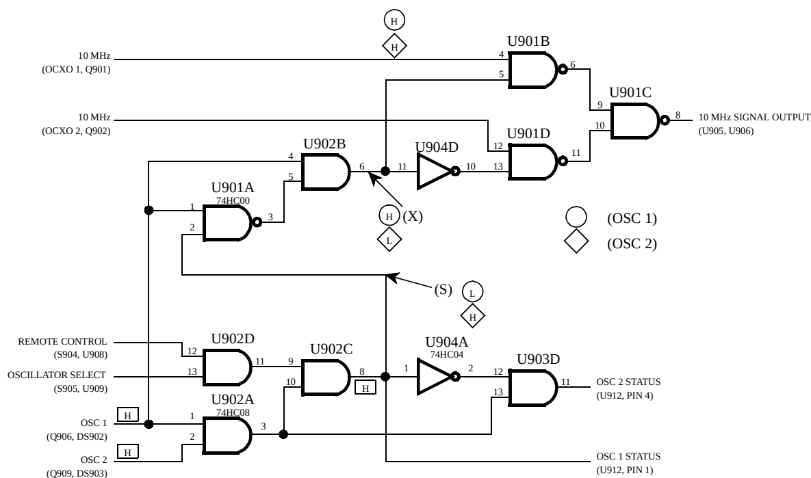
Figure 6-7 OCXO SWITCHING
