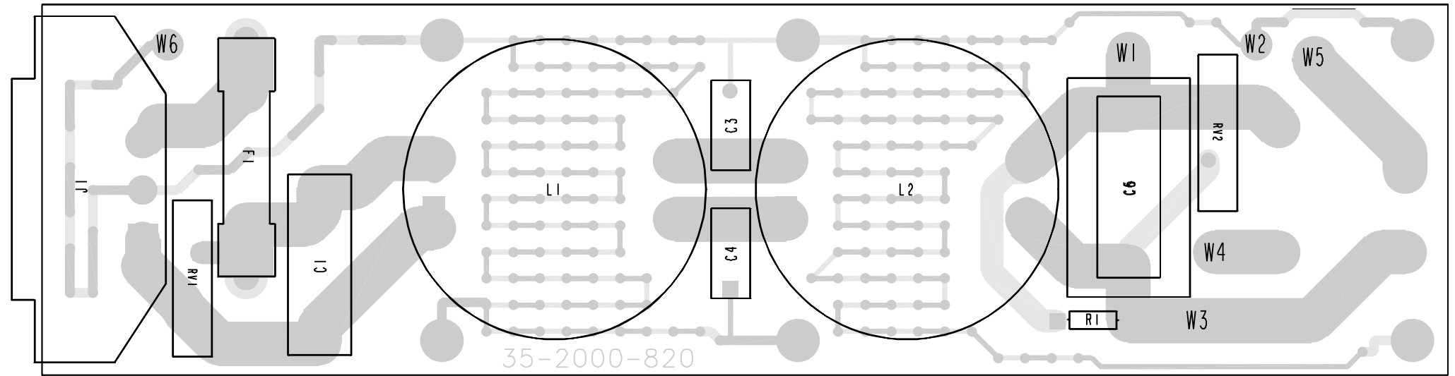
POWER SUPPLY FILTER BOARD COMPONENT LAYOUT FIGURE 10-48
