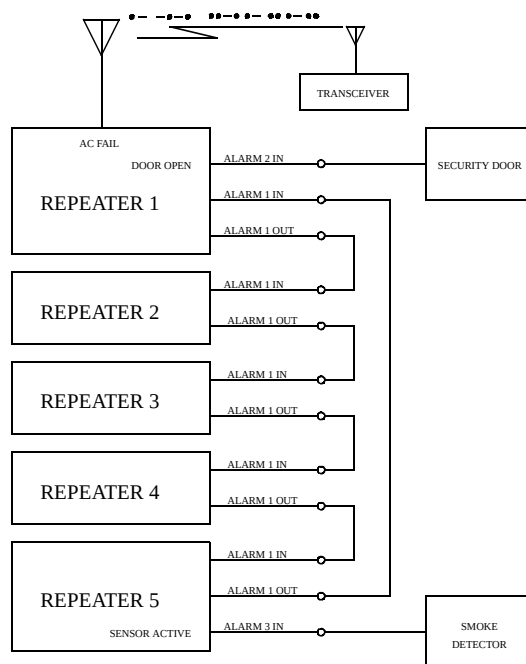
Figure 6-18 S500-S503
