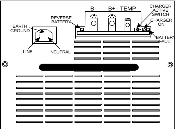
Figure 2-1 2000 SERIES POWER SUPPLY
