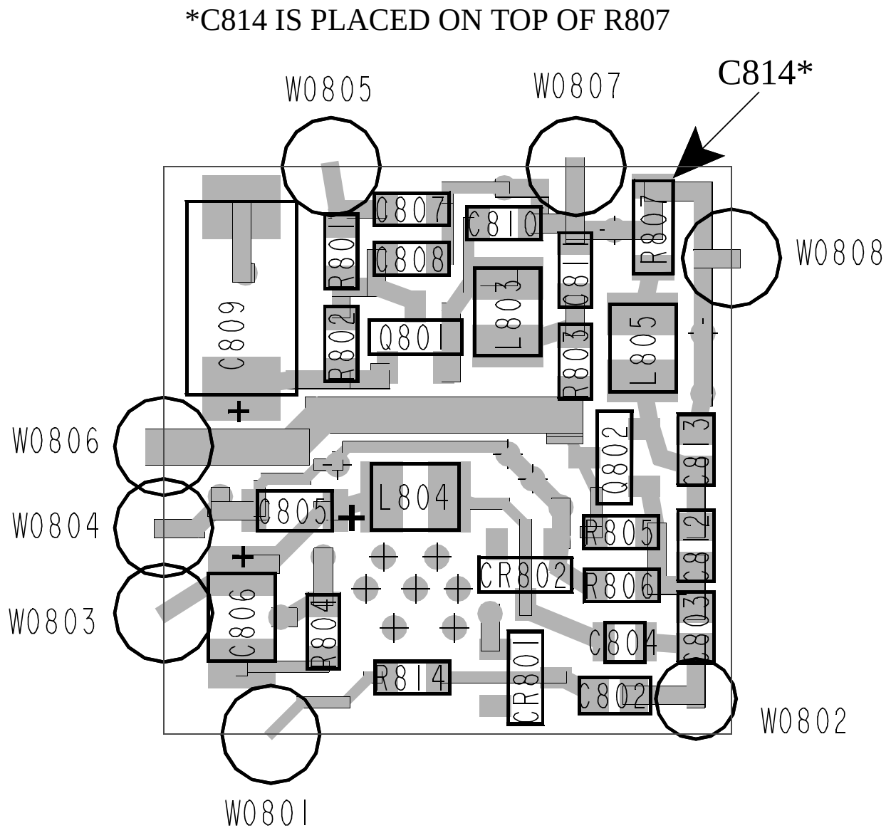
Figure 10-18 TRANSMIT VCO COMPONENT LAYOUT
