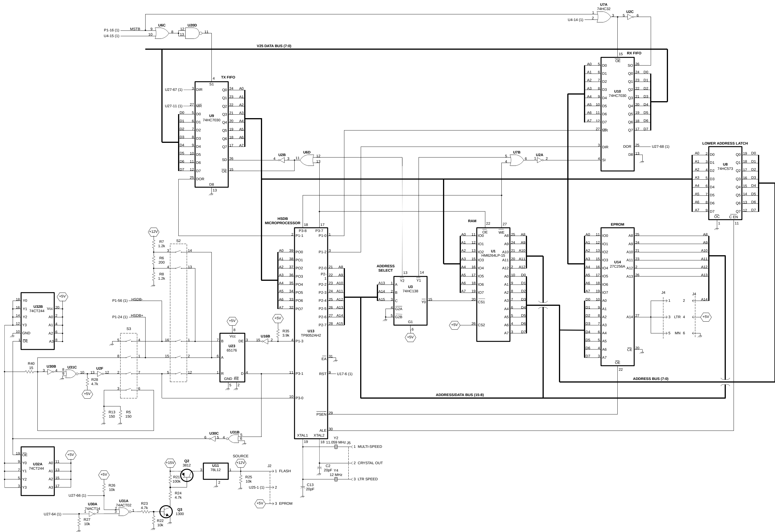
MAIN PROCESSOR CARD SCHEMATIC (2 OF 2) FIGURE 10-33
