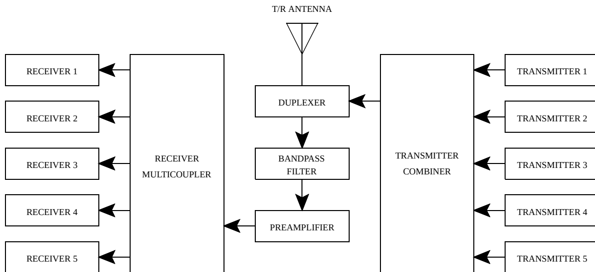
Figure 2-4 5-CHANNEL COMBINING SYSTEM
