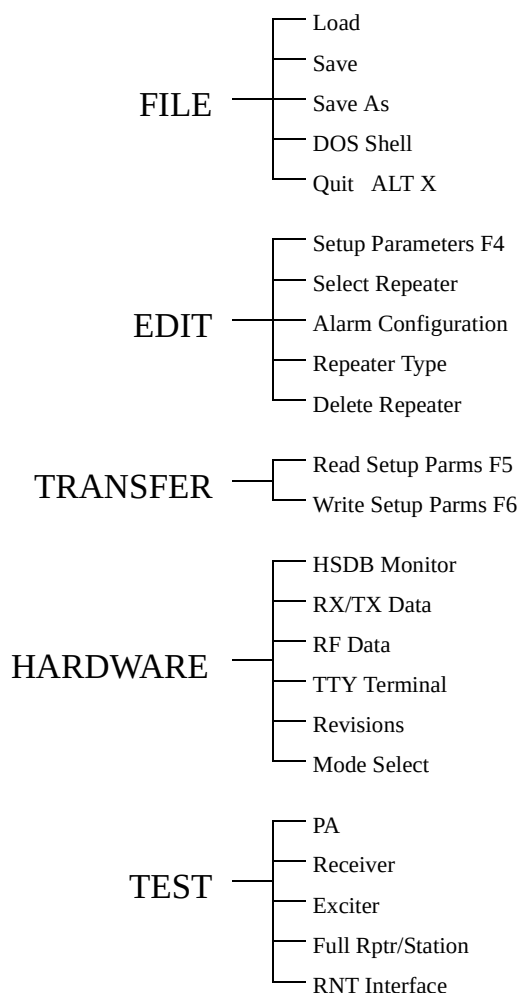
Figure 3-2 PROGRAMMING FLOWCHART
