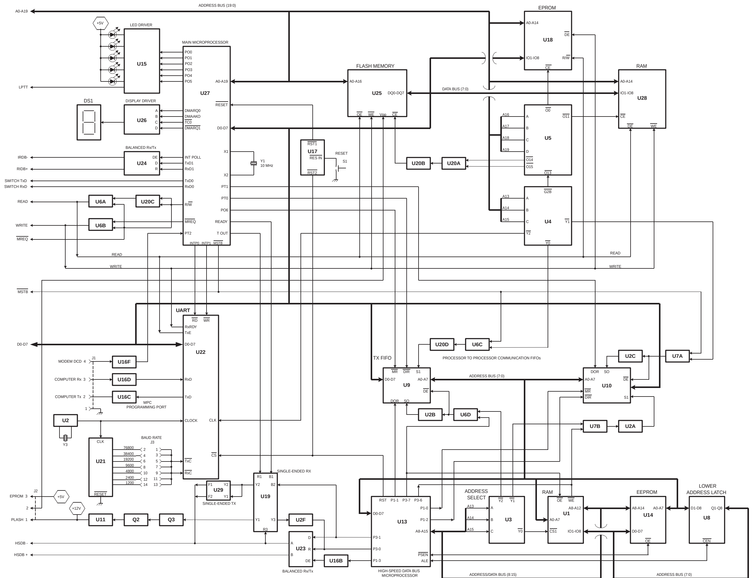
MAIN PROCESSOR BLOCK DIAGRAM FIGURE 6-20
