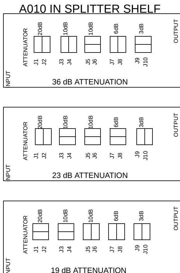
Figure 2-9 ATTENUATOR SETTINGS
