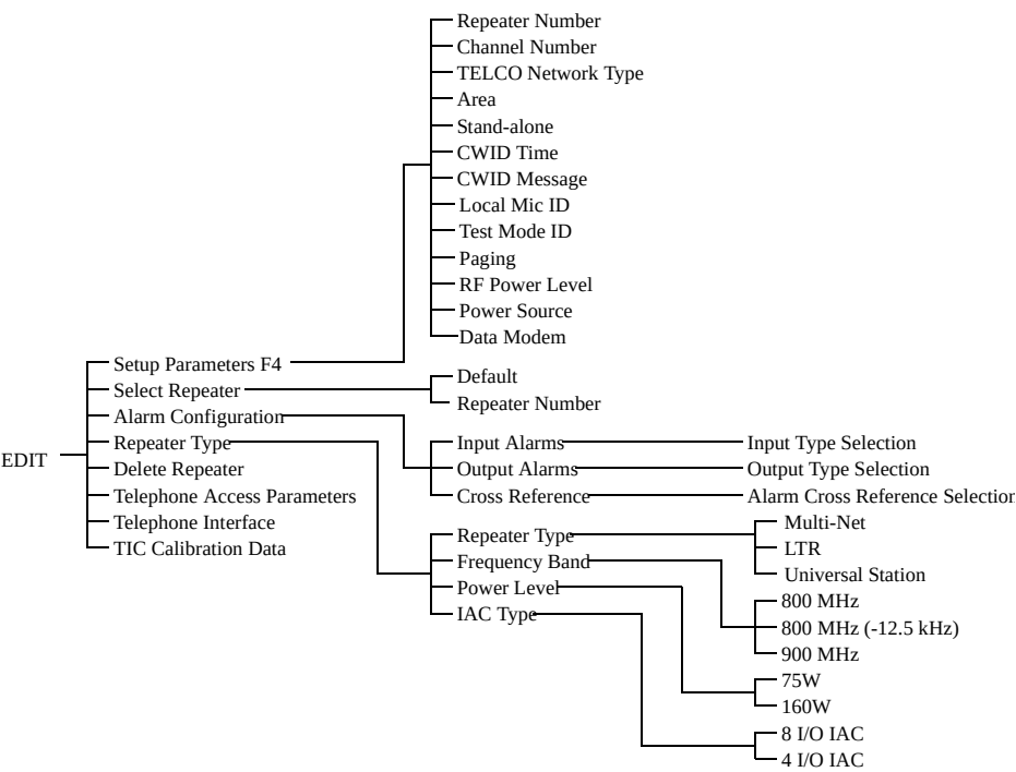
Figure 4-4 EDIT PROGRAMMING FLOWCHART
