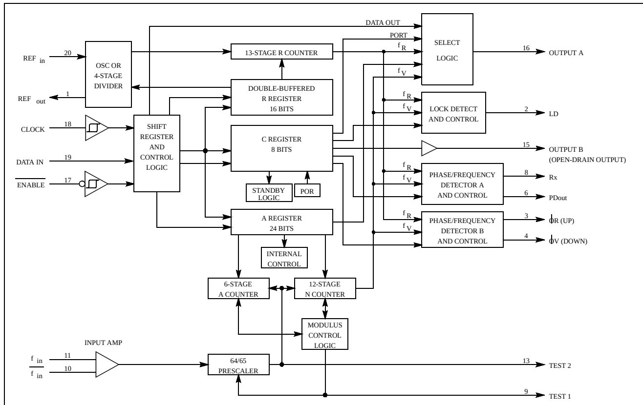
Figure 6-3 SYNTHESIZER BLOCK DIAGRAM
