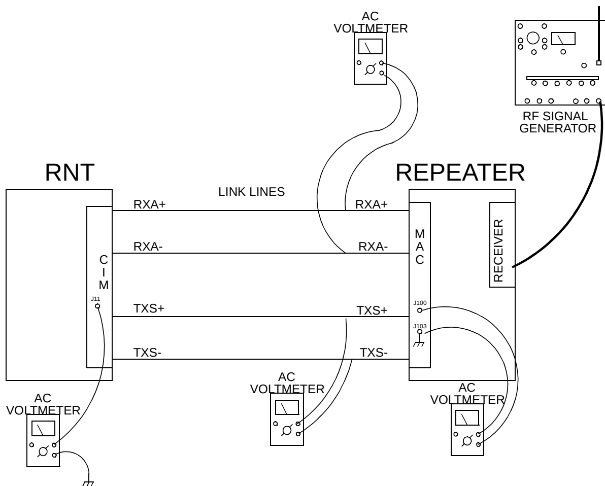
Figure 7-7 REPEATER TO CIM TEST SETUP
