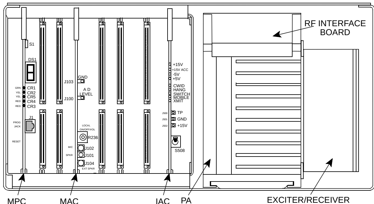
Figure 1-1 REPEATER CARDS
