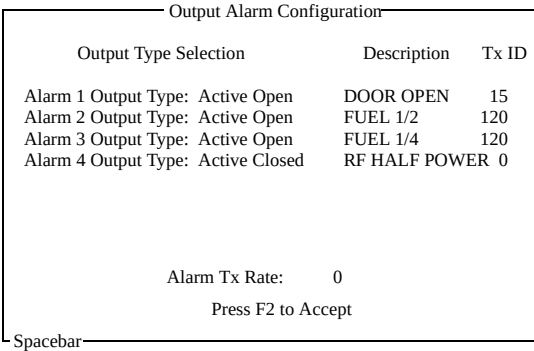
Figure 4-9 OUTPUT ALARMS
