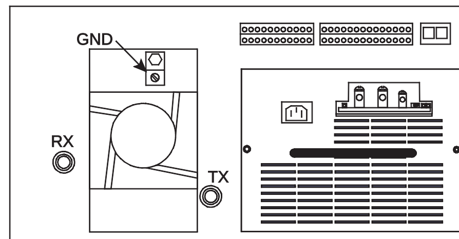
REPEATER REAR VIEW FIGURE 10-4
