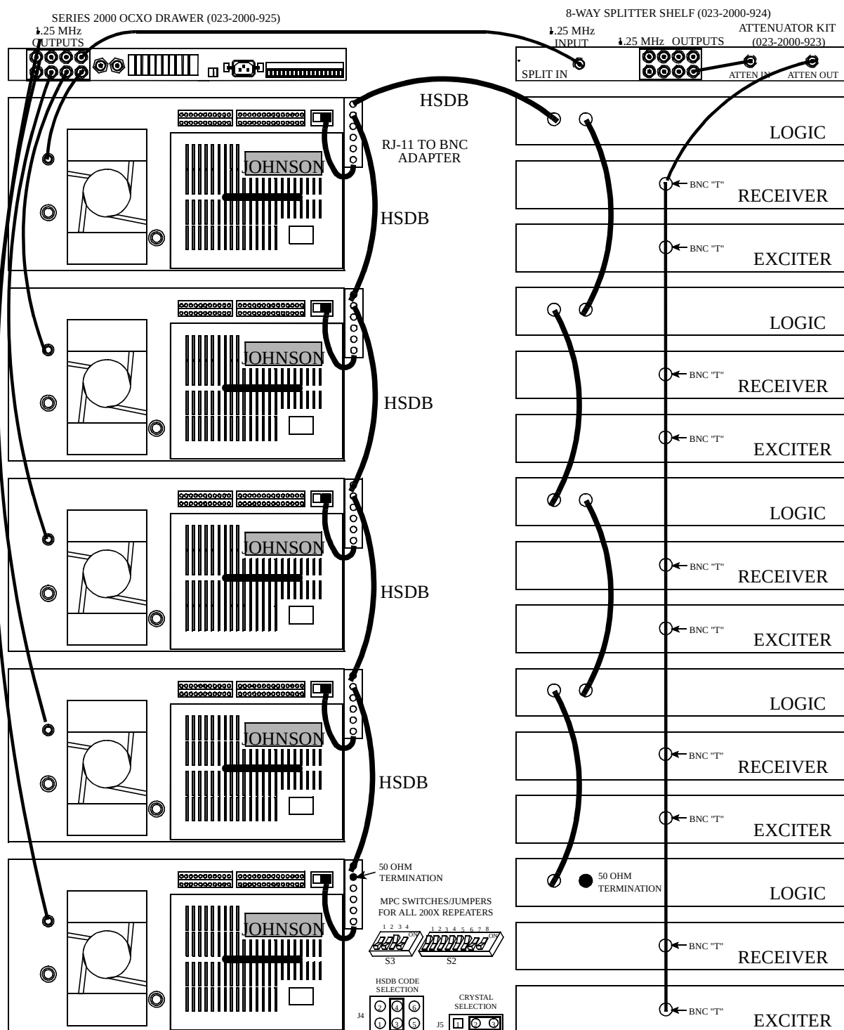
Figure 2-13 MIXED REPEATERS WITH 2000 OCXO DRAWER
