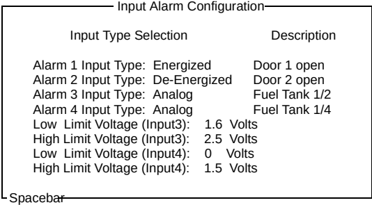
Figure 4-8 INPUT ALARMS
