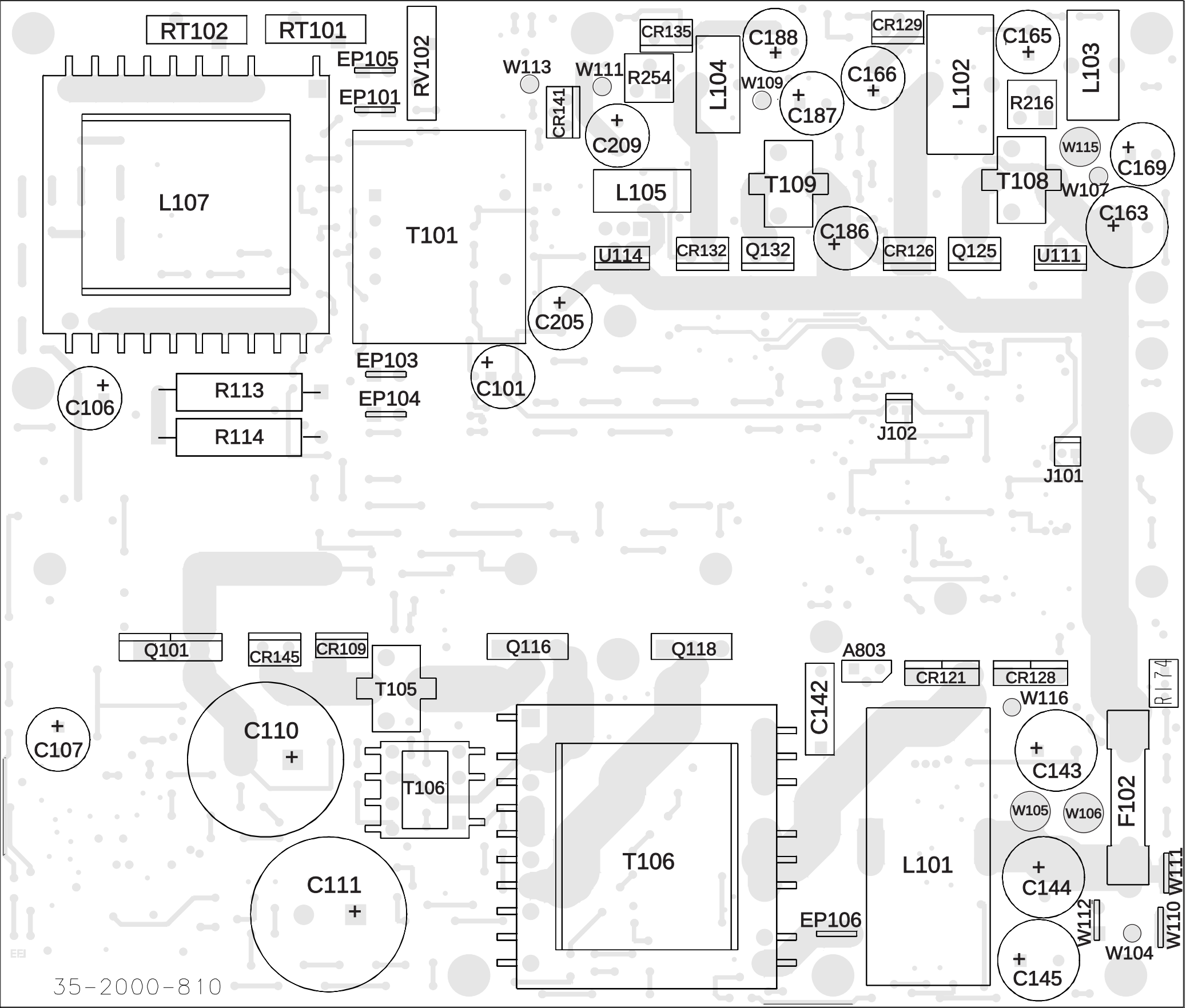
800W POWER SUPPLY COMPONENT LAYOUT (COMPONENT SIDE VIEW) FIGURE 10-45
