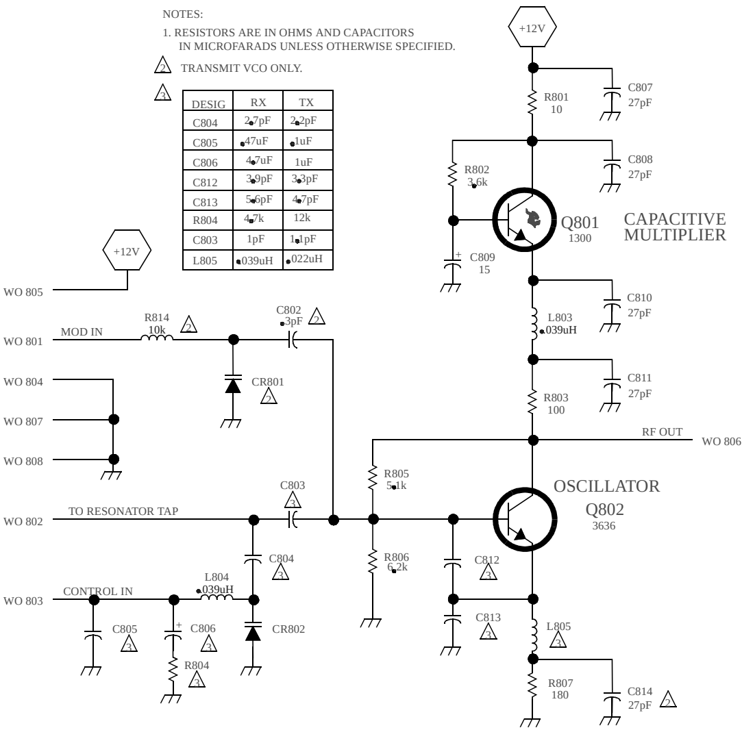
Figure 10-15 RECEIVE VCO SCHEMATIC
