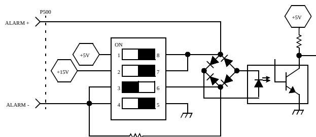
Figure 6-18 S500-S503
