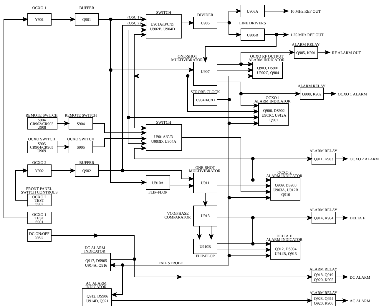
Figure 6-5 OCXO DRAWER BLOCK DIAGRAM
