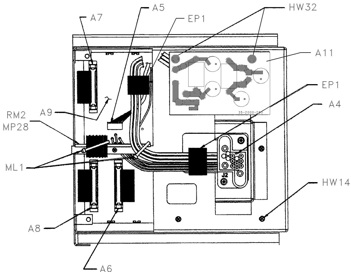
Figure 6-13 BACKPLANE CONNECTORS
