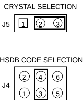
Figure 2-6 MPC JUMPERS
